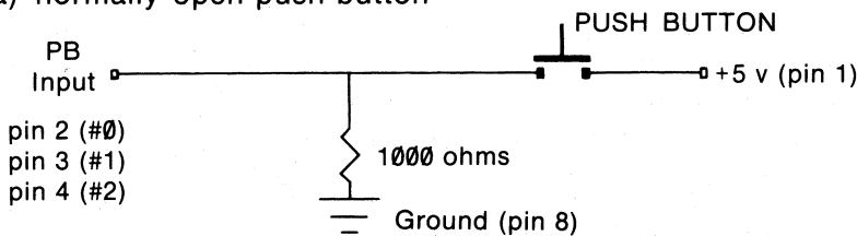
(a) normally-open push button
