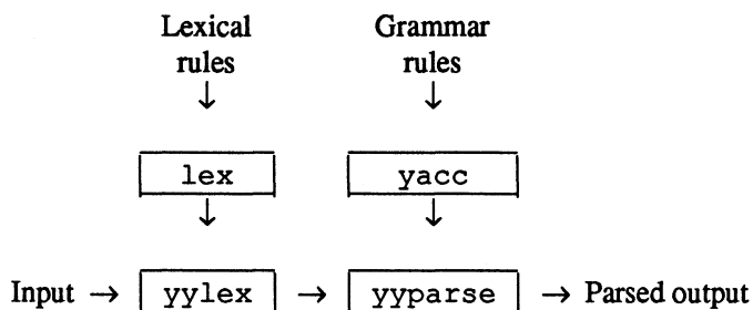
Figure 19-2. lex with yacc
